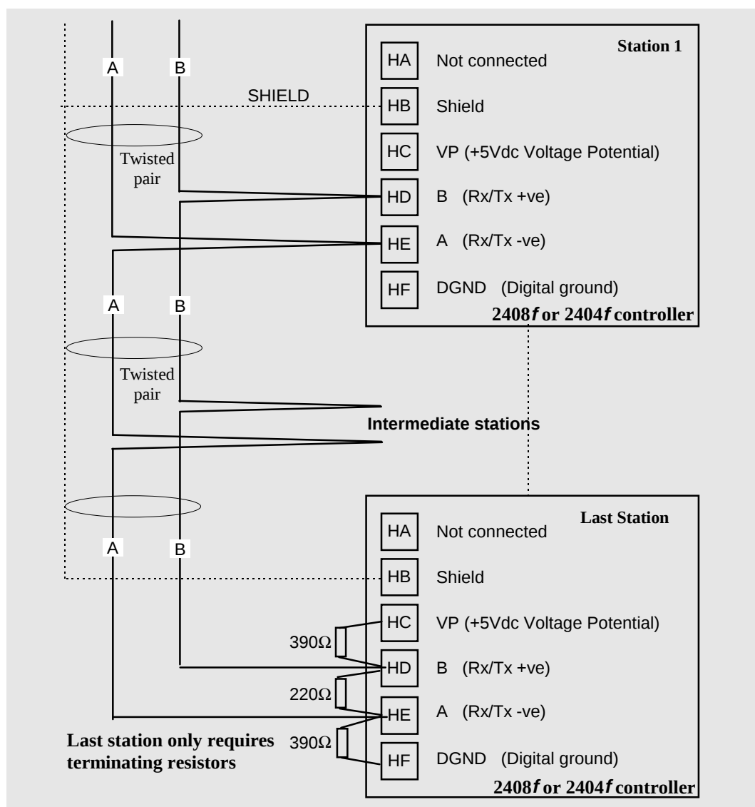
Figure 3-1: Connection Diagram for up to 32 Slaves.
